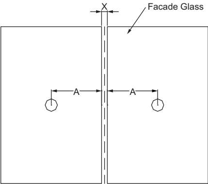
Glass Preparation for Façade Glass :
