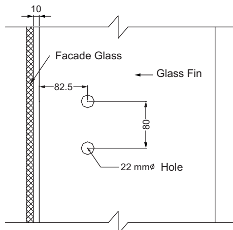
Articulated Bolts
