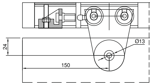
Roller Clamp Design : 80 kg Capacity
