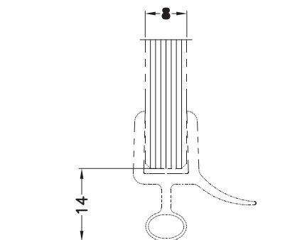
Soft Nose Seal XL - C 5009 / 8028
