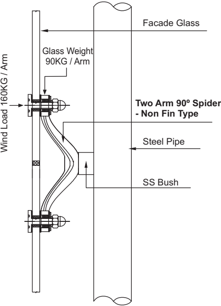
Section
