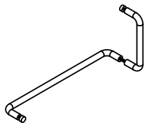
Towel Rod with Handle 458 x 205 x 18 mm Ordering Code : XL - C 8021A Reference Code : 9138089
