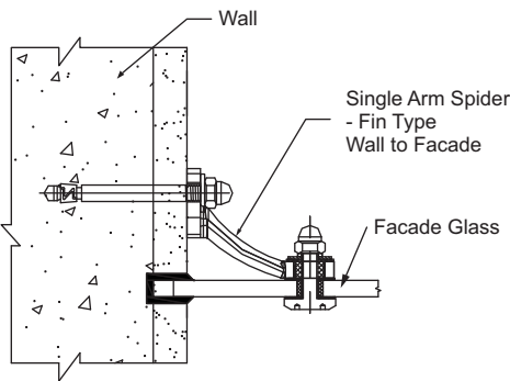
Plan - Option 2
