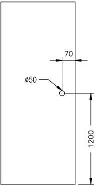
XL - C 3002A (D Type Handle - 300 x 22 mm)
