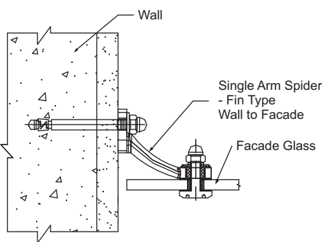
Plan - Option 2
