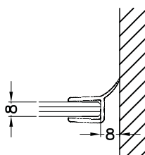
Wall Seal XL - C 5008 / 8030
