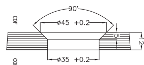
Countersunk Cutout Detail for XL - C 4115 & XL - C 4116
