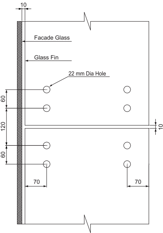
Fixed Bolt
