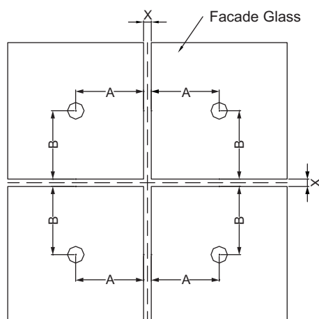
Glass Preparation for Façade Fins :
