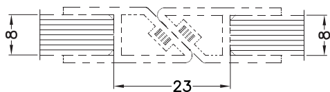
Magnetic Seal 180° XL - C 5013 / 8023 / 8026
