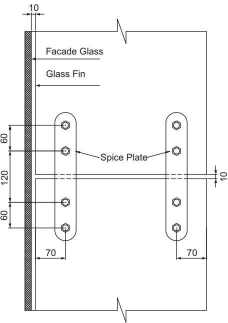
Fixed Bolt
