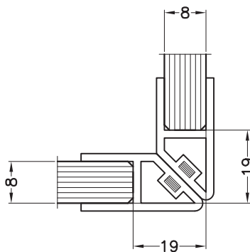
Magnetic Seal 90° XL - C 5012 / 8022 / 8025
