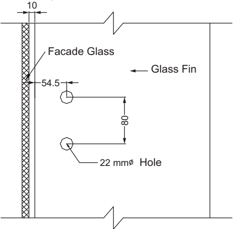
Fixed Bolts
