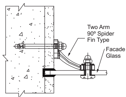
Plan - Option 2
