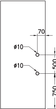
XL - C 3004A (D Type Handle - 600 x 30 mm)
