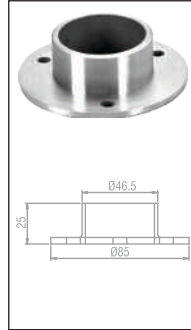
MWFHR-42.4 (S.S.316) AMWHR-42.4 (S.S.304) Wall Flange for Handrail
