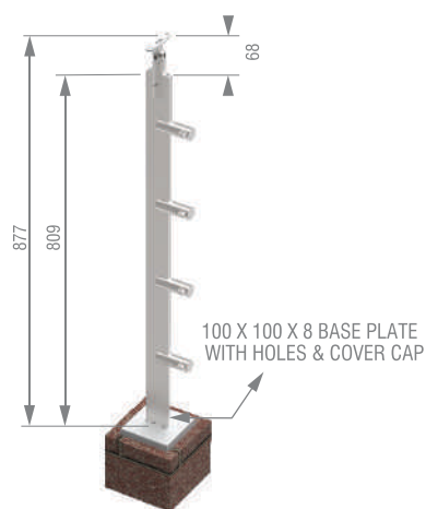
Top Mounted Flat (Hollow) Baluster with Horizontal Members
