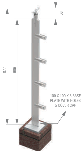
Top Mounted Flat Baluster with Horizontal Members
