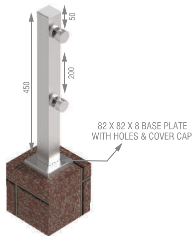
Top Mounted Square (Short) Baluster System With Glass - 40x40x450x1.5mm (DT32-1-GLS)
