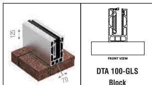
Top Mounted Hollow Aluminum System DTA100-GLS (Continue System)
