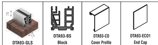
Top Mounted Rectangle Aluminum System DTA93-GLS / DTA91-GLS (Block Cover System)
