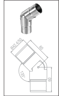
MBHRS-42.4/50 (S.S.316) AMBHR-42.4/50 (S.S.304) Smooth Bend for Handrail
